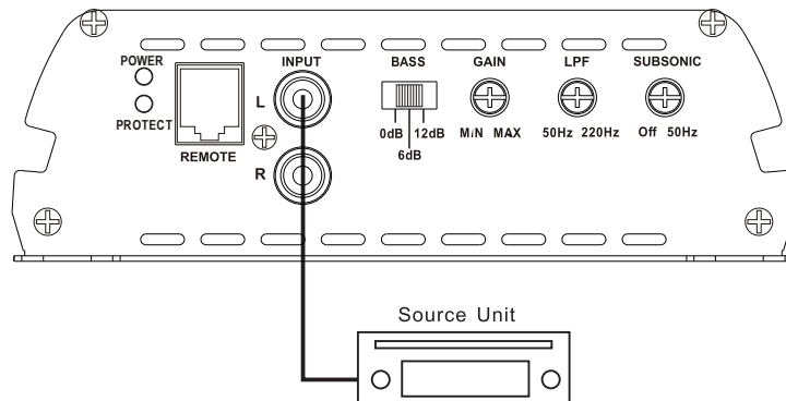
VL1500D FRONT PANEL
